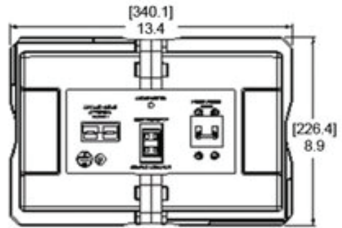
Maximum dimensions in [mm] inches
